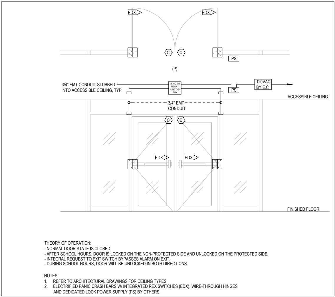
4 DOUBLE DOOR - EXIT DEVICE - UNLOCK ONLY SCALE: NONE
